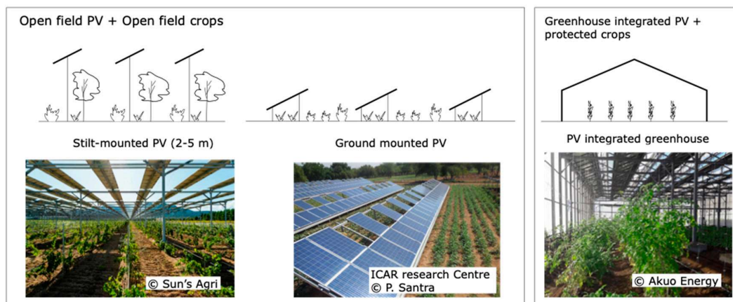
Figure 12. Agrivoltaic systems: typologies.
