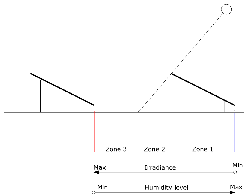
Figure 9. Ground-mounted PV and crop zones (adapted from [145]).
