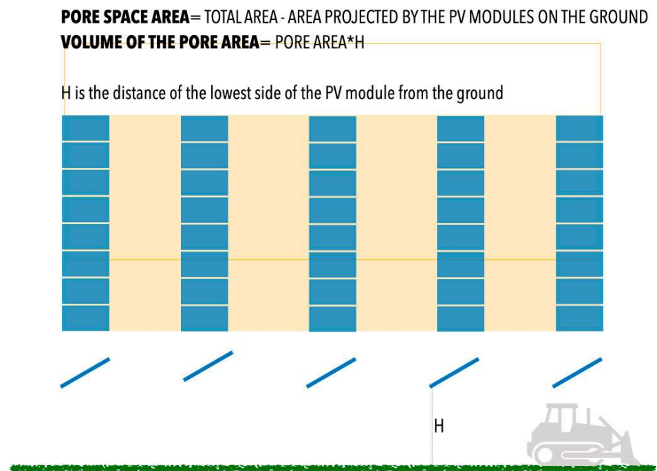
Figure 14. The three-dimensional pattern of the APV systems.
