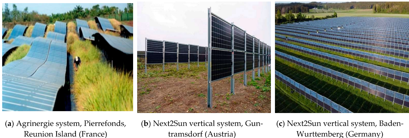
Figure 7. Commercial plants with ground-based PV mounting system. © Akuo Energy (a), Next2Sun GmbH (b,c).
