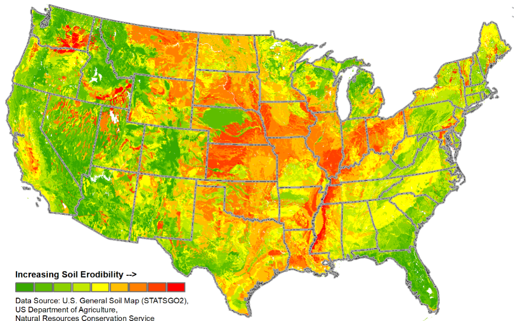
Figure 2. Soil Erodibility in the Contiguous U.S.
