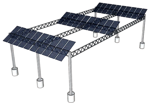
Fig. 47: Illustration of different system types oriented east-west, south and south-east. © Fraunhofer ISE
