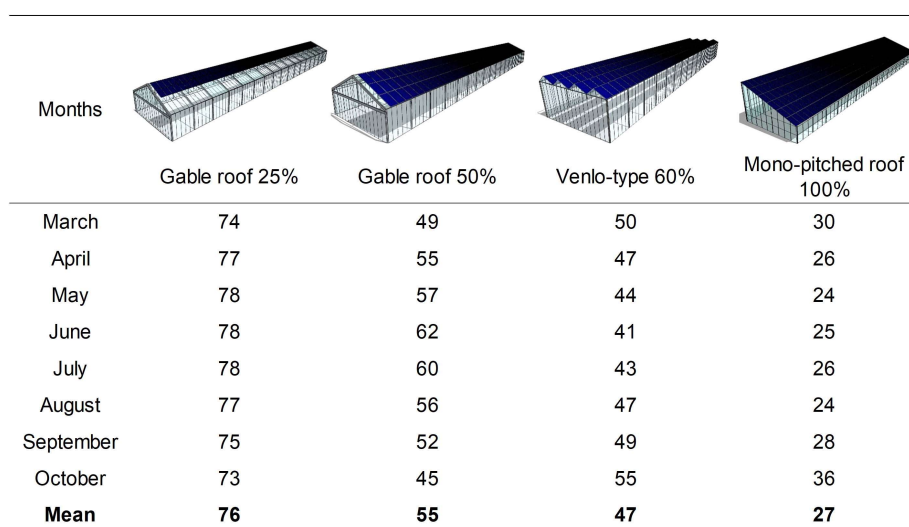
FIGURE 2 | Average monthly percentage of available cumulated PAR from March to October compared with a conventional greenhouse without PV panels on the roof, expressed as GGR coefficients for four photovoltaic greenhouse (PVG) types with E-W orientation. The coefficients were calculated at 1.5 m above ground level and retrieved from the literature (Cossu et al., 2018).
