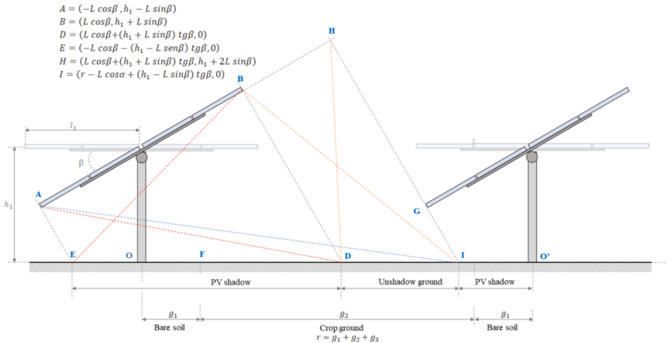
Fig. 4. APV system geometry to calculate view factor coefficients in two surfaces of infinite lengths, upon the surface is shadow/unshadow and bare soil/crop.
