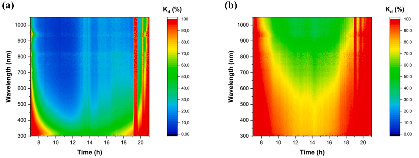
Fig. 8. Diffuse fraction coefficient ( k_d ) calculated for a) clear sky, and b) hazy sky.
